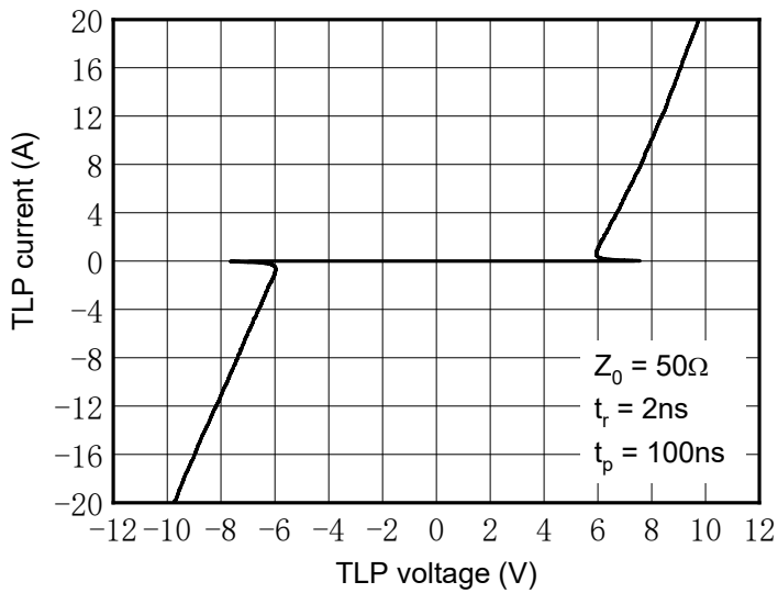
Fig. 9 TLP Measurement
