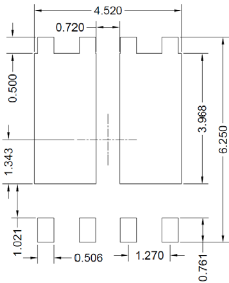
Suggested Solder Pad Layout Top View
