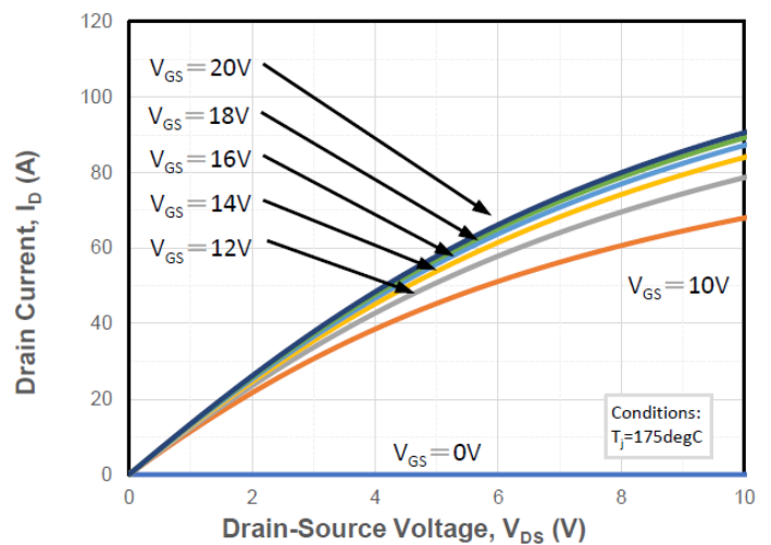
Figure 2. Output Characteristics T_j = 175^\circ C
